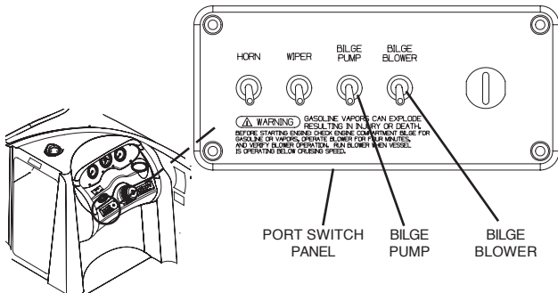
BILGE PUMP AND BILGE BLOWER SWITCH (FIG. 4.1.3)
