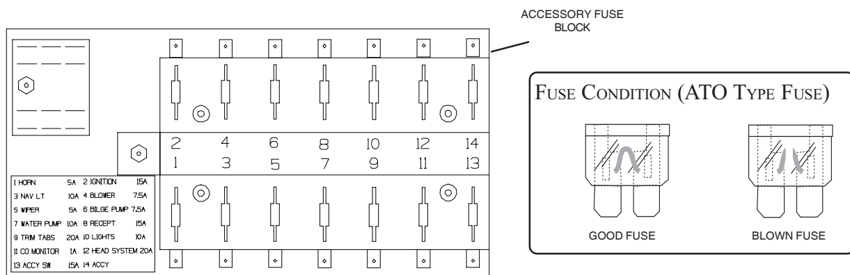
FUSES SIZES (FIG. 6.4.2)
