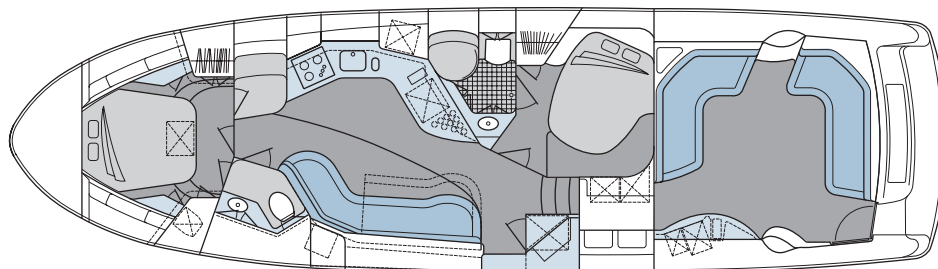
Cabin/Cockpit Layout
