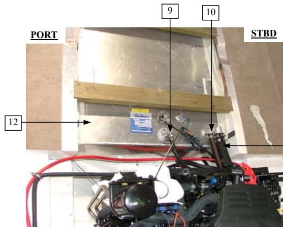
AFT ENGINE WELL FACING FORWARD
