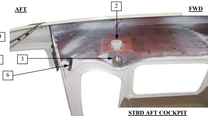
STBD AFT COCKPIT
