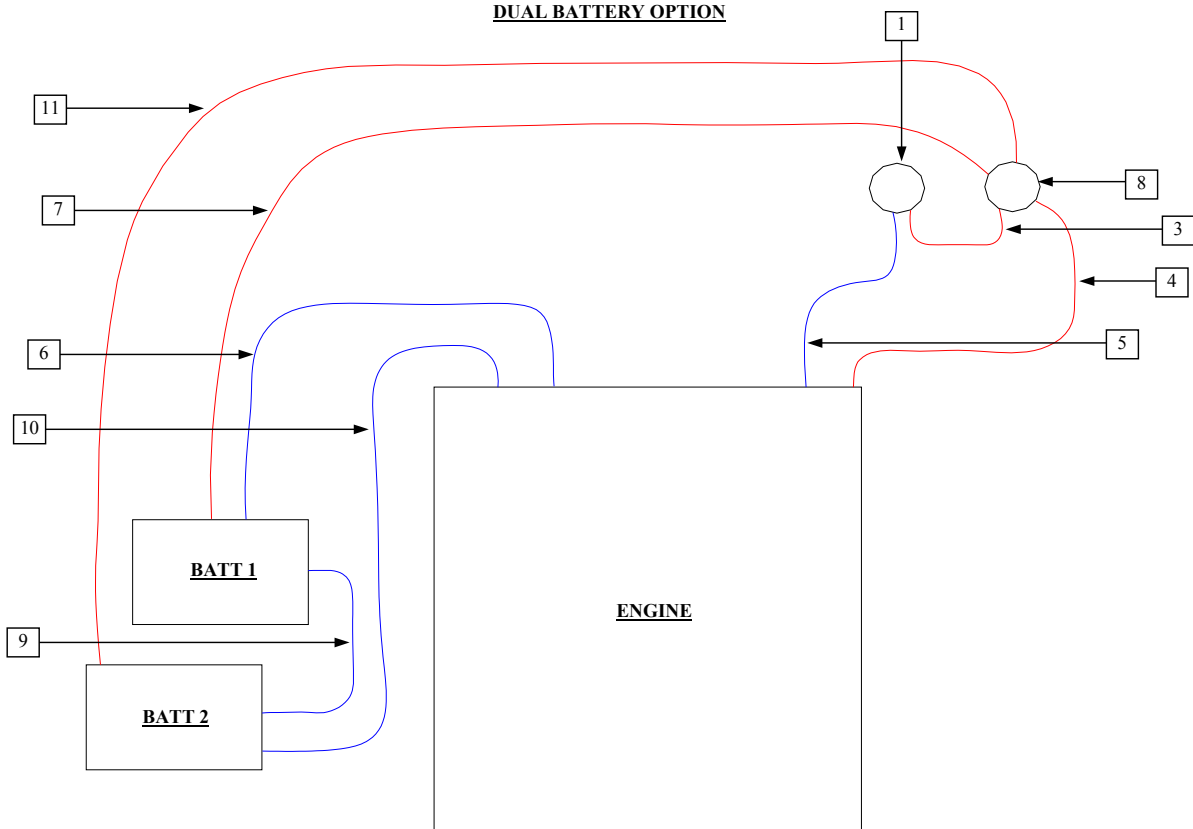
DUAL BATTERY OPTION
