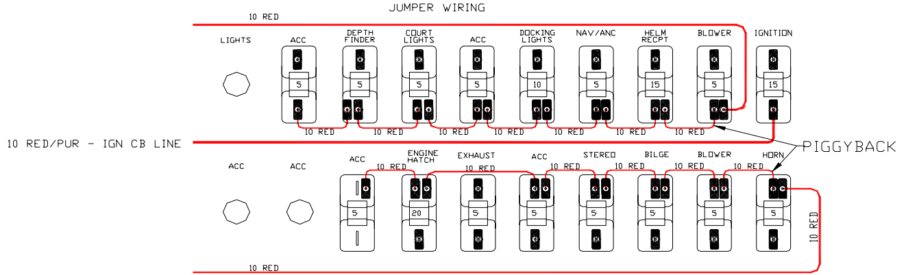
205-00299-A & 205-00300-A CIRCUIT BREAKER PANELS
