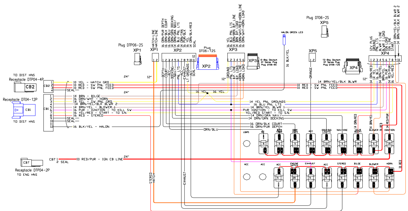
205-00299-A & 205-00300-A CIRCUIT BREAKER PANELS
