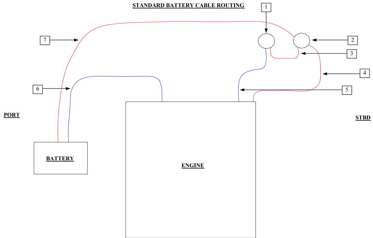
STANDARD BATTERY CABLE ROUTING
