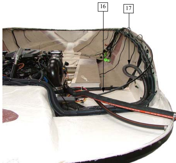
STBD AFT ENGINE WELL FACING FORWARD
