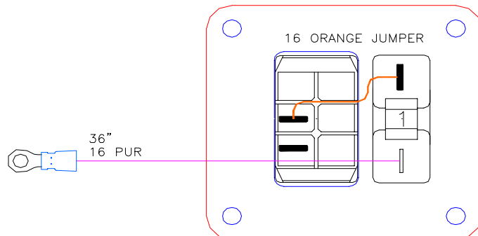
205-00164 SE NEUTRA SALT PANEL
