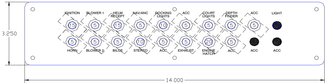
205-00299-A & 205-00300-A CIRCUIT BREAKER PANELS
