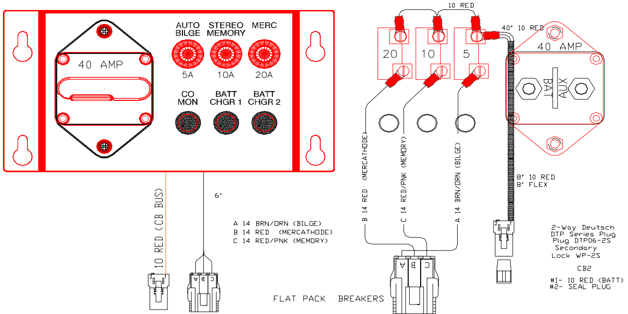
205-00106-A BILGE BREAKER BOX ASSEMBLY
