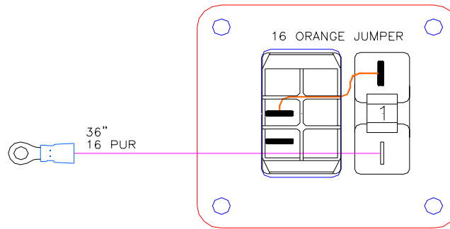
205-00164 SE NEUTRA SALT PANEL
