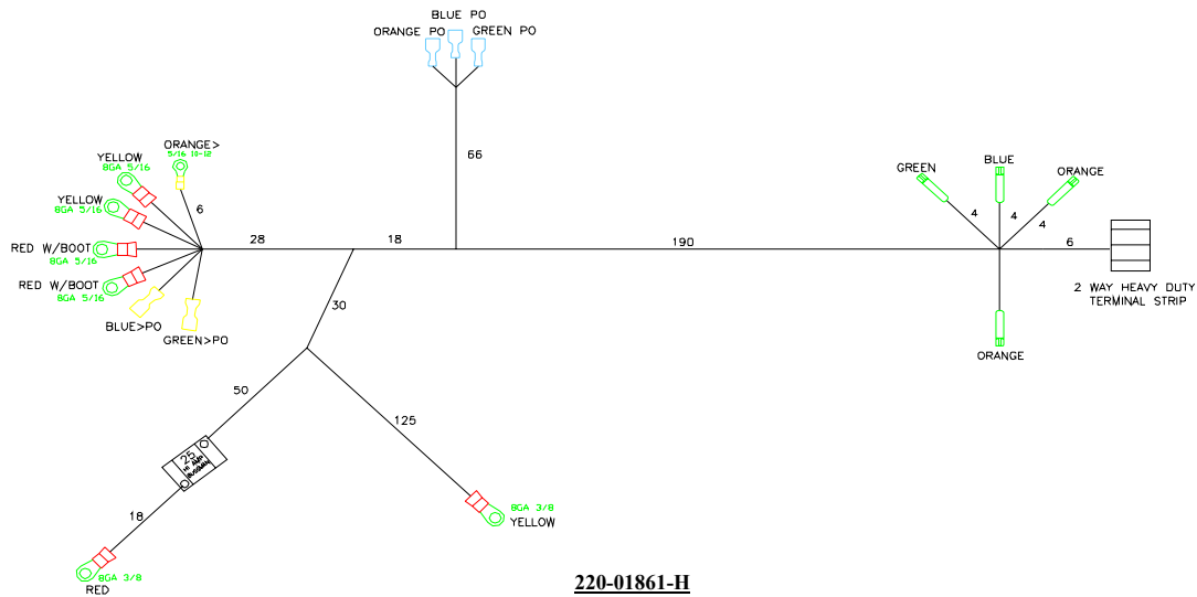
220-01861-H WINDLASS HARNESS
