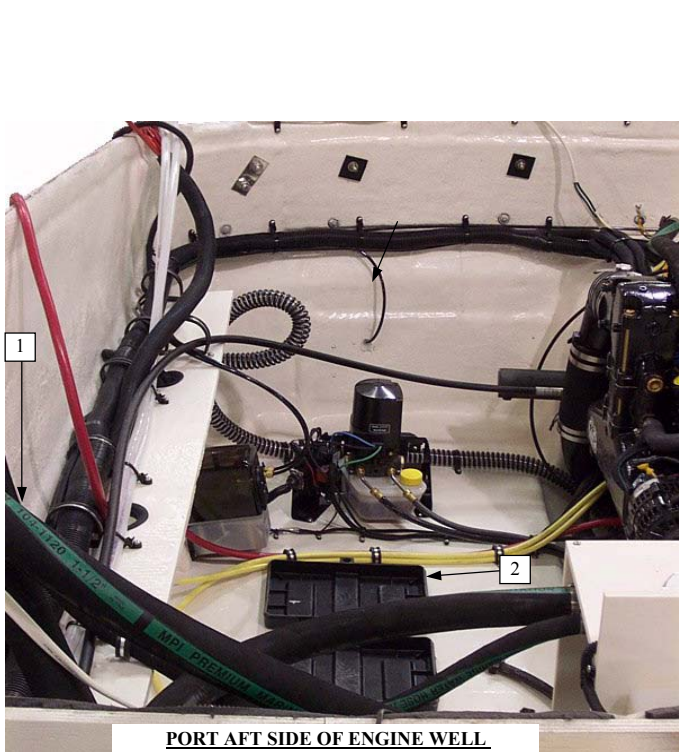
PORT AFT SIDE OF ENGINE WELL
