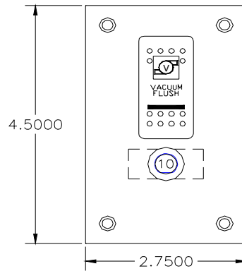
205-00206-A VACUUM FLUSH PANEL
