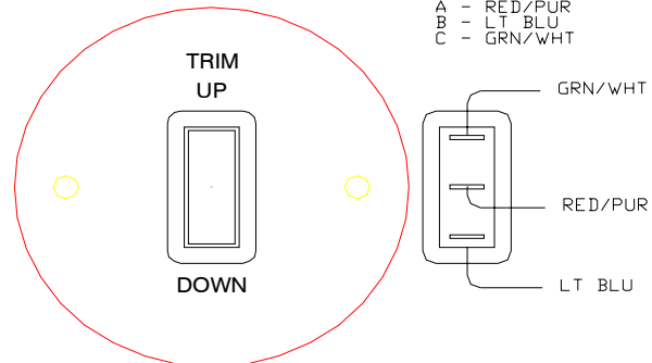
205-00203-A SE TRANSOM TRIM PANEL (MERCURY)
