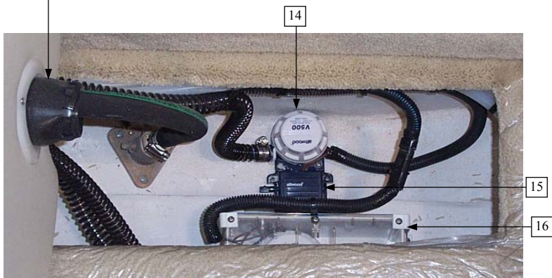
SUMP PUMP AND FORWARD BILGE
