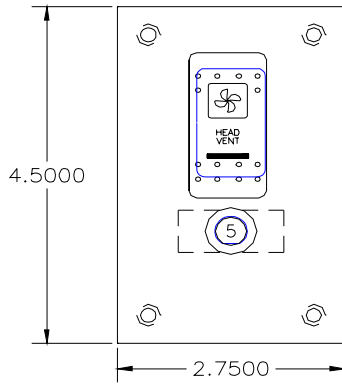
221-03329-P HEAD VENT PANEL
