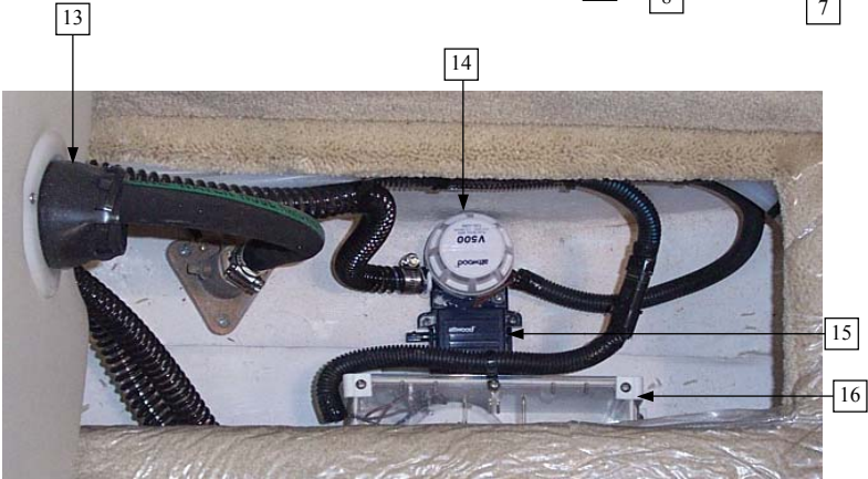
SUMP PUMP AND FORWARD BILGE
