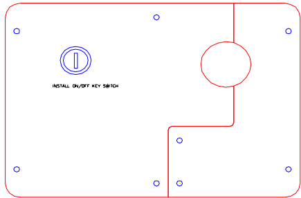
230-01665-K SPLIT MACERATOR PANEL KIT
