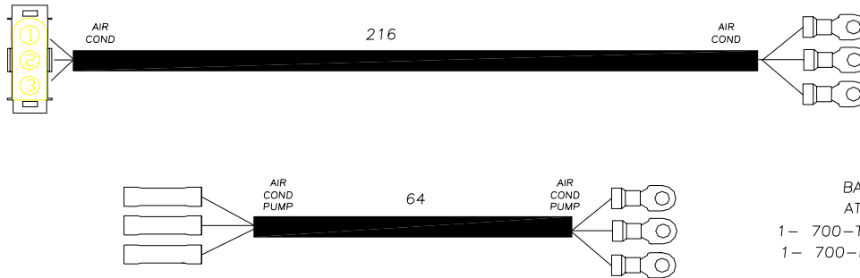
220-01873-H AIR CONDITIONER HARNESS
