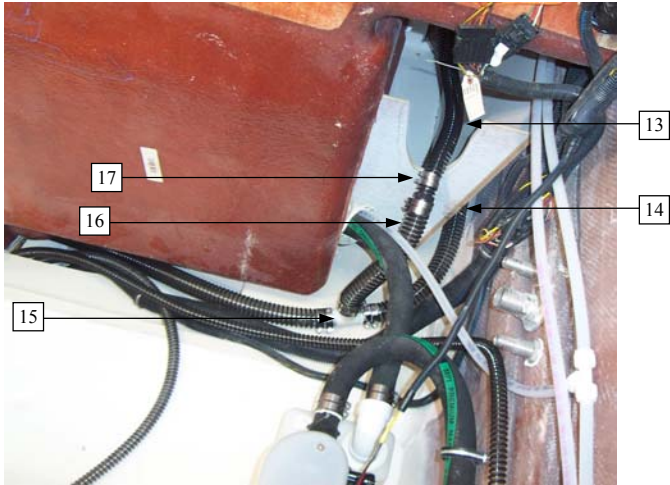
GRAY WATER
