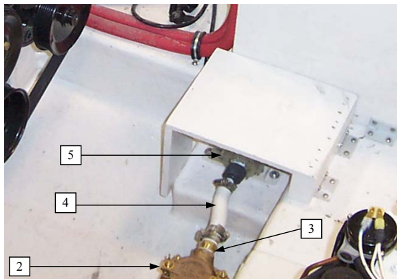
AIR CONDITIONING SYSTEM IN ENGINE WELL
