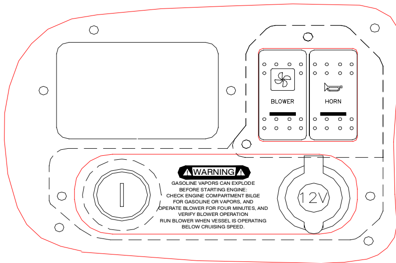
205-00198-A SUNESTA PORT SWITCH/IGNITION PANEL
