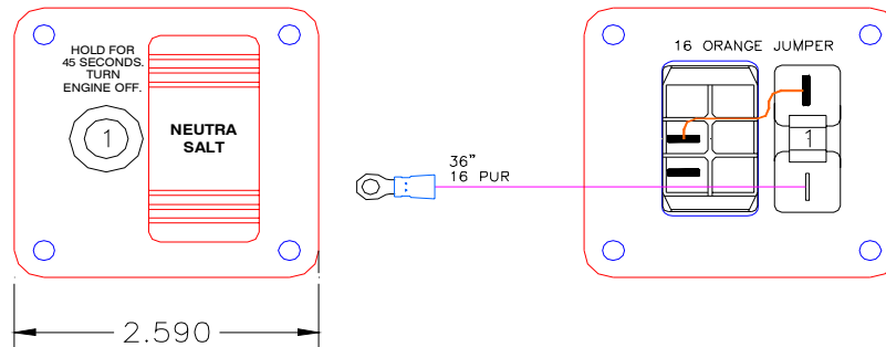
205-00164 SE NEUTRA SALT PANEL
