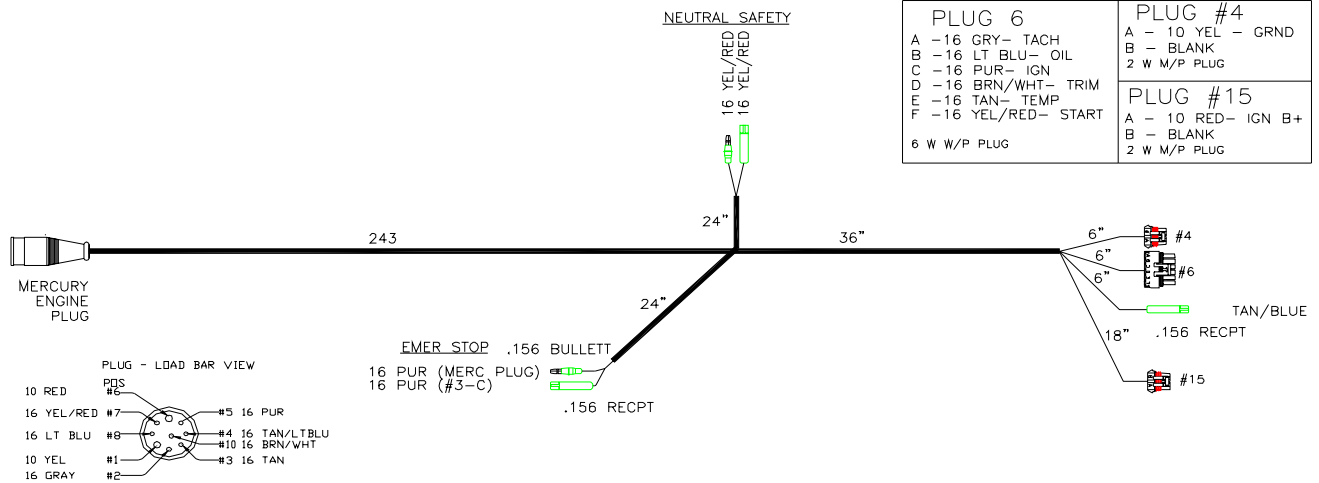
203-00148-A 274 SUNESTA ENGINE HARNESS
