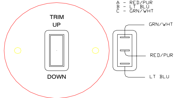
205-00203-A SE TRANSOM TRIM PANEL (MERCURY)
