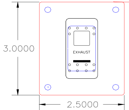
205-00233-A QUICK & QUIET EXHAUST PANEL
