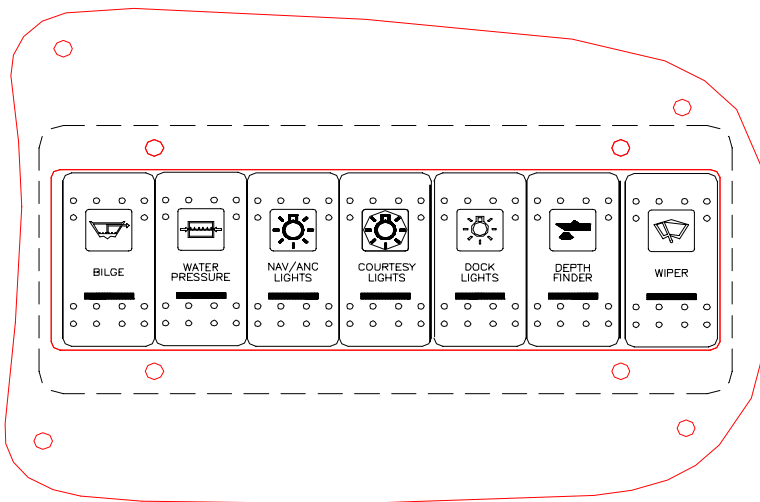
205-00199-A SUNESTA STBD SWITCH PANEL
