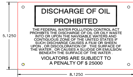
210-00518-F OIL DISCHARGE FACEPLATE
