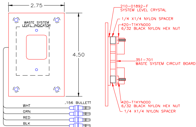
205-00149-A WASTE LEVEL PANEL
