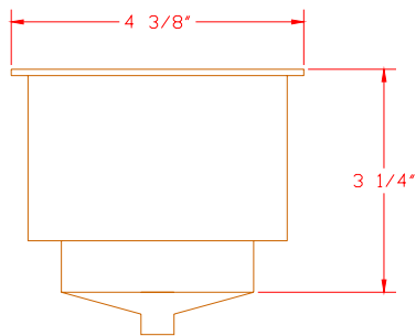
10-399 4X3 W/ DRAIN TUBE COLOR MATCHED
