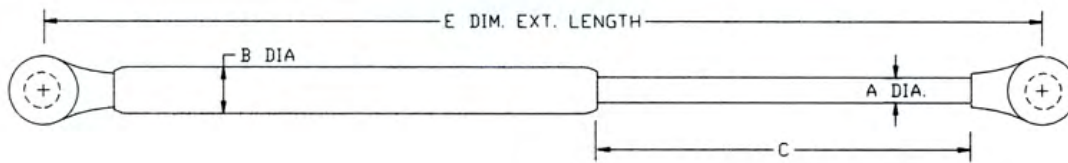
316 STAINLESS STEEL GAS SPRINGS 625 & 750 SERIES WITH COMPOSITE OR SS ENDS FIXED FORCE
