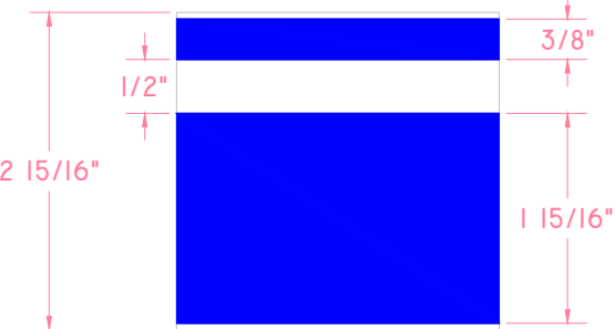
PART # 30-611
