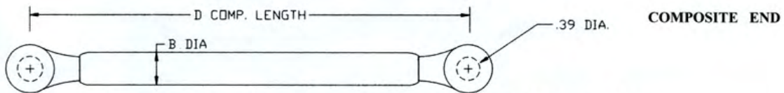
316 STAINLESS STEEL GAS SPRINGS 625 & 750 SERIES WITH COMPOSITE OR SS ENDS FIXED FORCE
