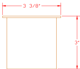
10-400 3" NARROW FLANGE
