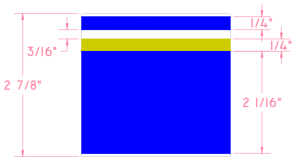
PART # 30-106
