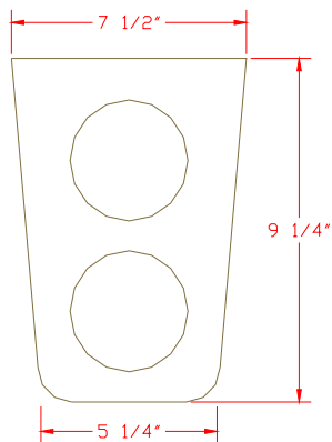
32-195 DOUBLE CUPHOLDER SMOKE PLEXI
