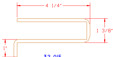
32-015 CUPHOLDER COLOR MATCHED
