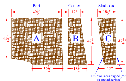
Aft Berth Cushions Grady-White Part Number 20-101
