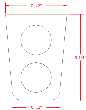
32-195 Double Cupholder Smoke Plexi
