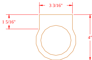
32-148 Cupholder Color Matched
