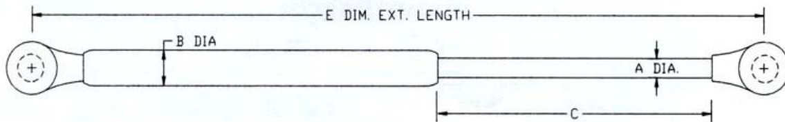
316 STAINLESS STEEL GAS SPRINGS 625 & 750 SERIES WITH COMPOSITE OR SS ENDS FIXED FORCE
