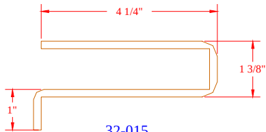
32-015 Cupholder Color Matched
