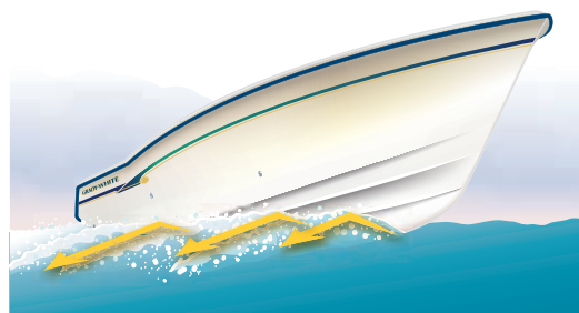
Strakes and chines knock down spray
