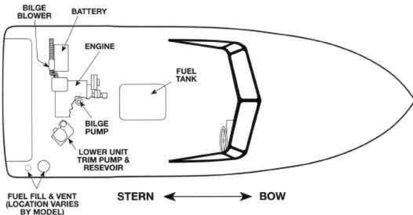
FIGURE 3.1 EQUIPMENT LOCATOR
