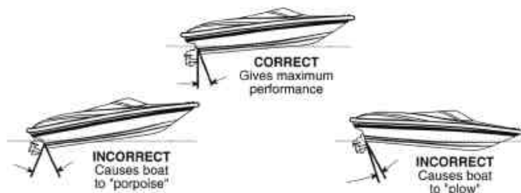
FIGURE 4.3 TRIMMING
