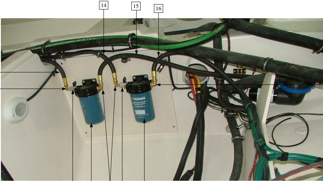
STARBOARD SIDE OF ENGINE WELL
