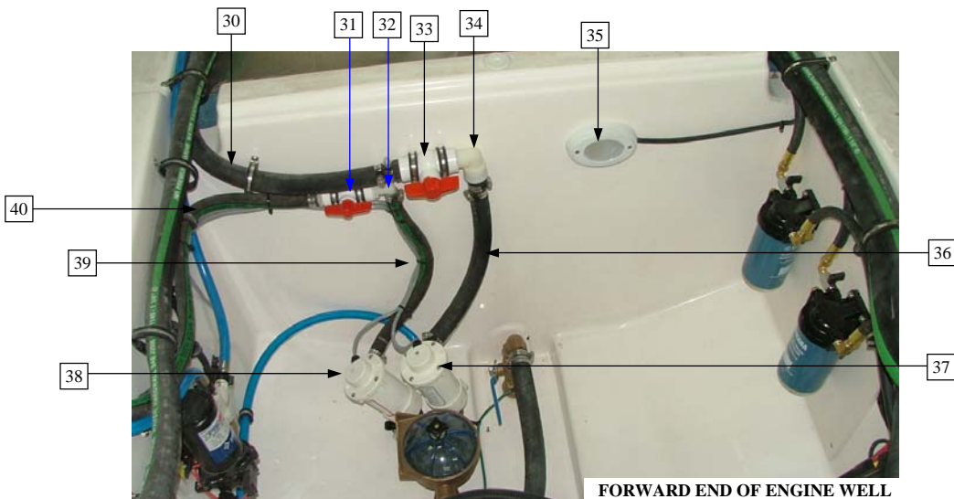
FORWARD END OF ENGINE WELL
