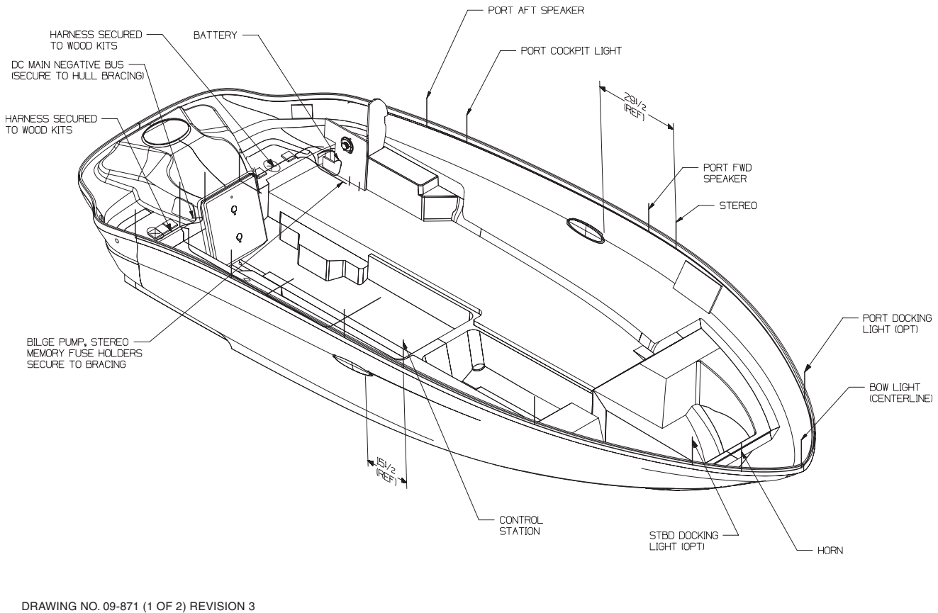
WIRE HARNESS (FIG. 6.8.1)
