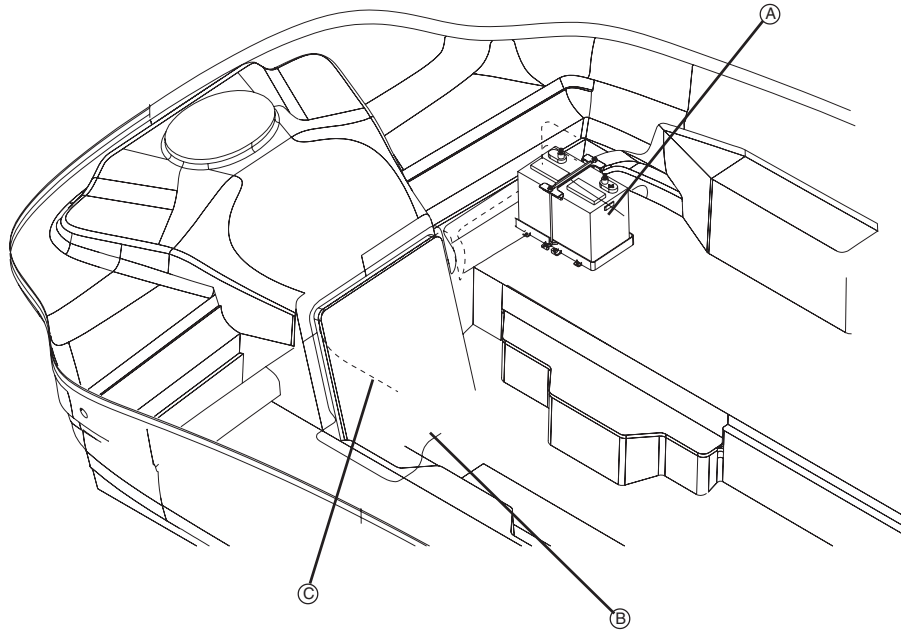
BATTERY CABLE ROUTING (FIG. 6.2.1)
