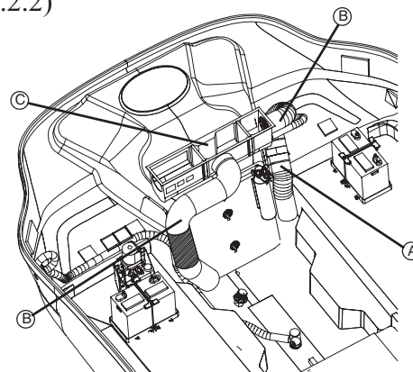
BILGE BLOWER (FIG. 4.2.2)
