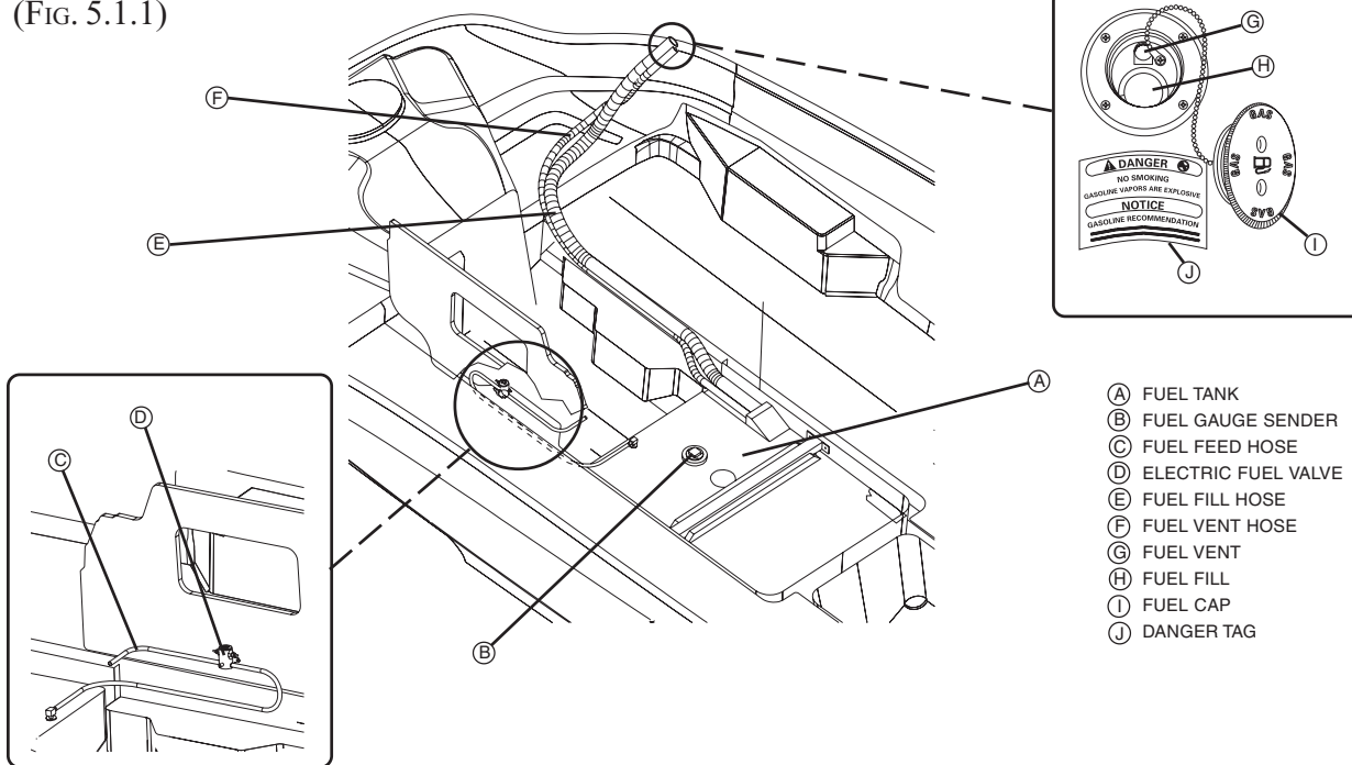
FUEL LINE ROUTING (FIG. 5.1.1)
