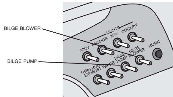
BILGE PUMP AND BILGE BLOWER SWITCH (FIG. 4.1.3)
