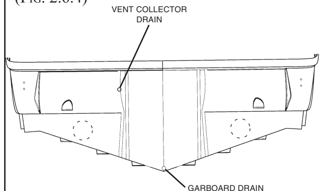
TRANSOM THROUGH-HULL CUTOUTS (FIG. 2.6.4)
