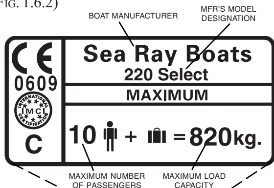
BUILDER'S PLATE (INTERNATIONAL) (FIG. 1.6.2)
