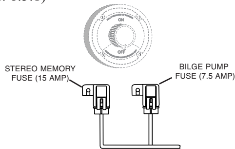
STEREO MEMORY/BILGE PUMP FUSES (FIG. 6.5.1)
