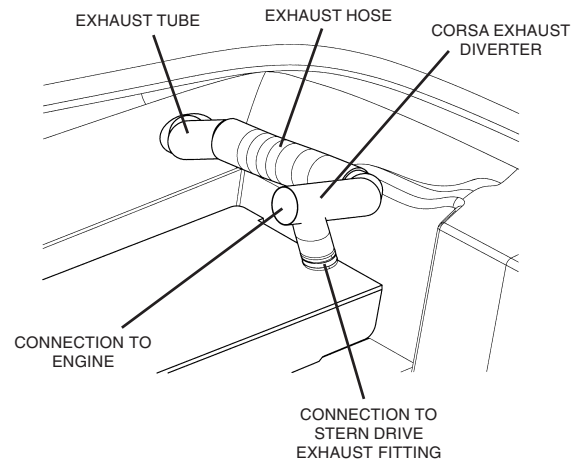
CORSA™ EXHAUST SYSTEM HOSE ROUTING (VIEW OF STARBOARD ASSEMBLY) (FIG.7.1.2)
