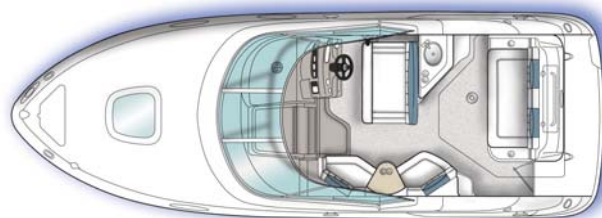
Cockpit Layout
