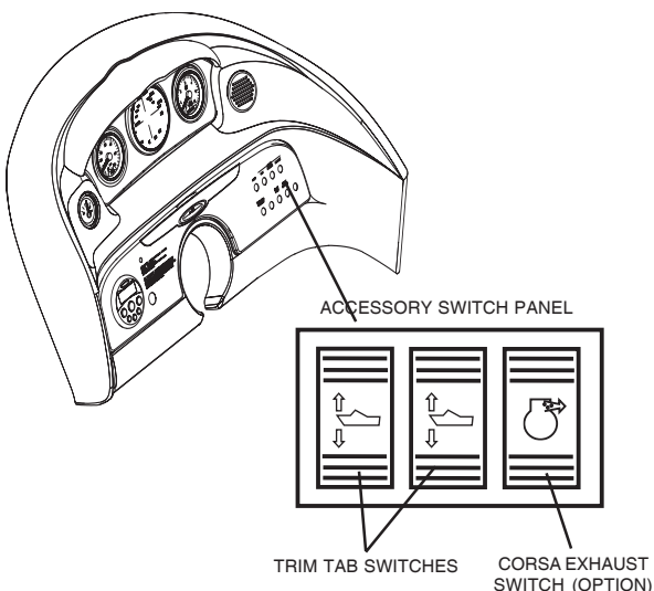
CORSA™ EXHAUST SYSTEM SWITCH (FIG.7.1.1)
