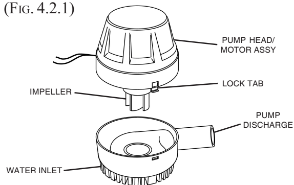
BILGE PUMP ASSEMBLY (FIG. 4.2.1)
