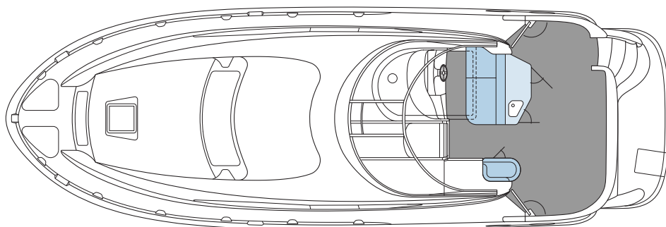
Cockpit Layout
