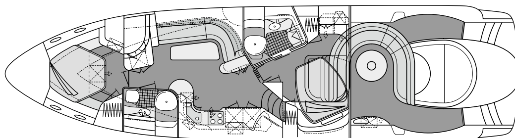
Cabin Layout w/Optional Garage
