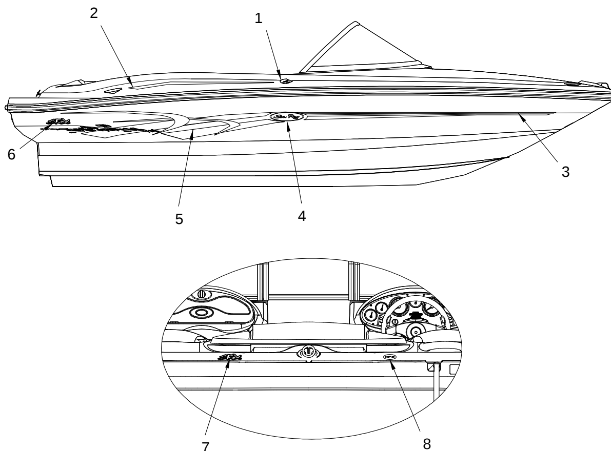
TRANSOM DETAIL
