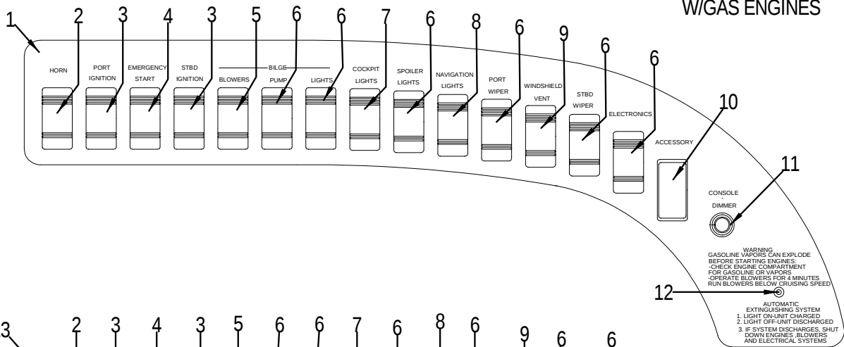
SWITCH PANEL W/GAS ENGINES
