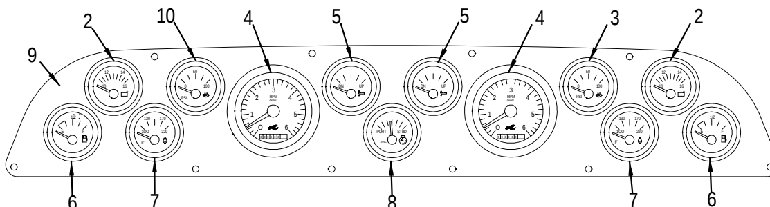
STERN DRIVE DIESEL ENGINE INSTRUMENT PANEL
