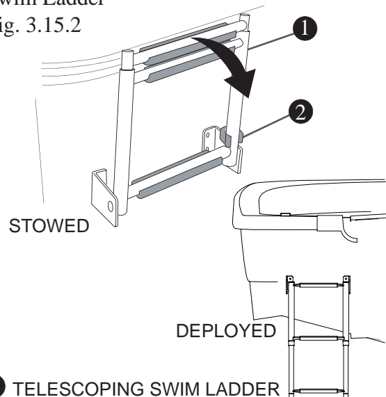
Swim Ladder
