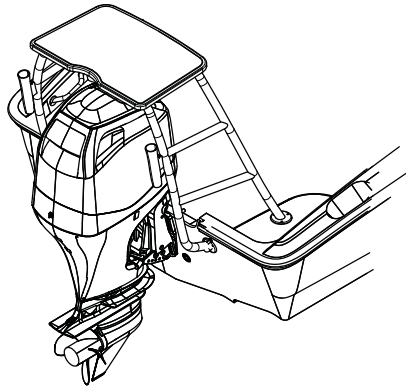
Poling Platform with Rodholders (Option) Fig. 3.13.1
