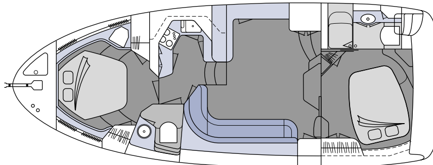
Floor plan
